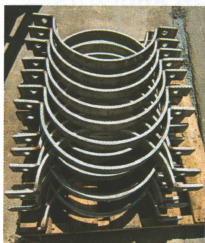
The J-D Shop custom fabricated (above) brackets for skimmers for Hubbard Construction's I-95 ABC and (left) brackets for suspending pipe along a Central Blvd bridge for Murphy Construction.
